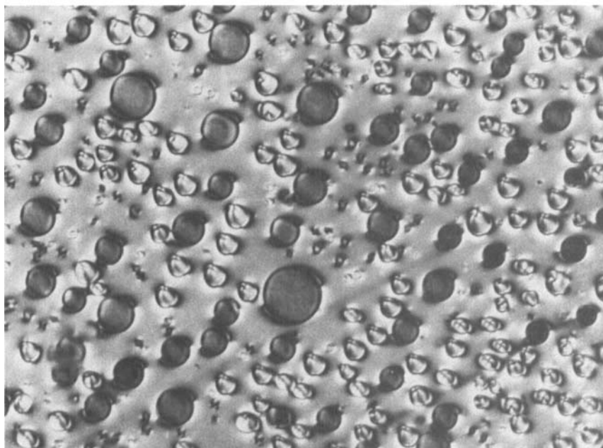
FIGURE 3a Coexistence of N_R and N_D phases in a mixture with 30 mol% of C_7OHBT at 88^\circ C . Sample taken between SiO coated plates and crossed linear polarizers ( \times 560 ). Notice that the point defects are present at the centers of relatively small N_R droplets.
