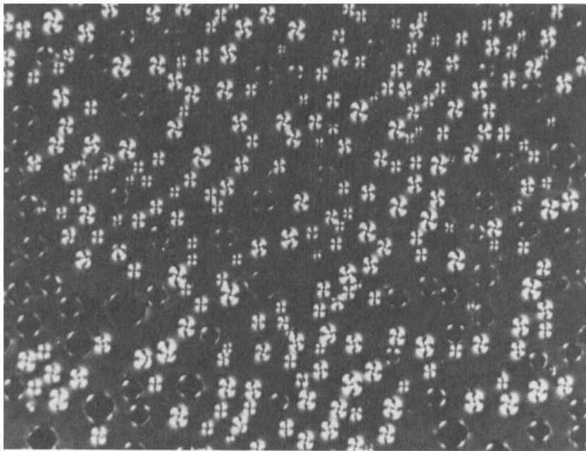
FIGURE 5 A coexistence region between N_R and N_D phases photographed between crossed linear polarizers with \psi = 0^\circ ( \times 570 ).
