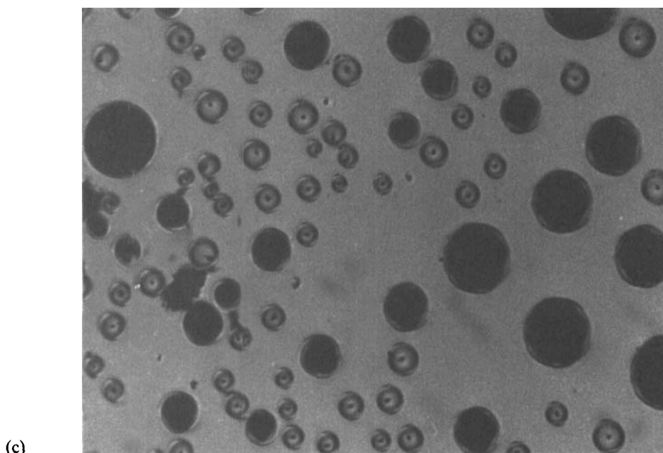
FIGURE 1c Same sample area as in Figure 1a between crossed circular polarizers ( \times 675 ).
