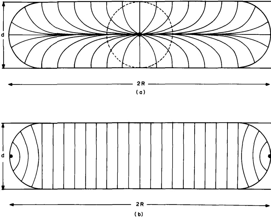
FIGURE 8a Vertical cross section of the director configuration of an N_R drop with a point defect of strength +1 in the center, with the director oriented homeotropically on the glass plates.
