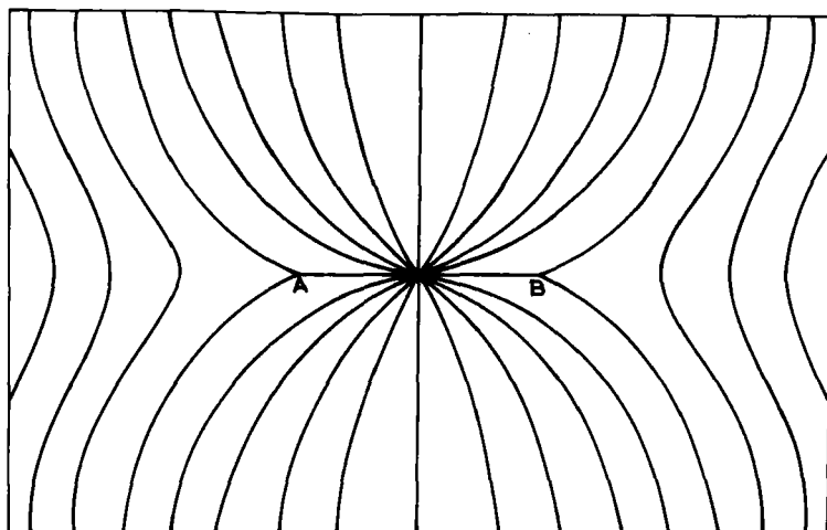
FIGURE 2 Schematic diagram of the director distortion around a point defect of strength +1 being annulled by a singular ring of strength -1 . The singular ring intersects the paper at points A and B.
